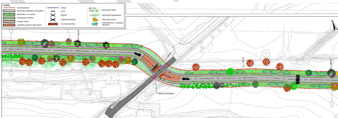
Figure 4-6 Excerpt from Figure WCGW-ROD-HGN-S1_ML-DR-CH-200504 from Volume 3 illustrating how the proposed development will divert around an existing dwelling and cross the L2018.
