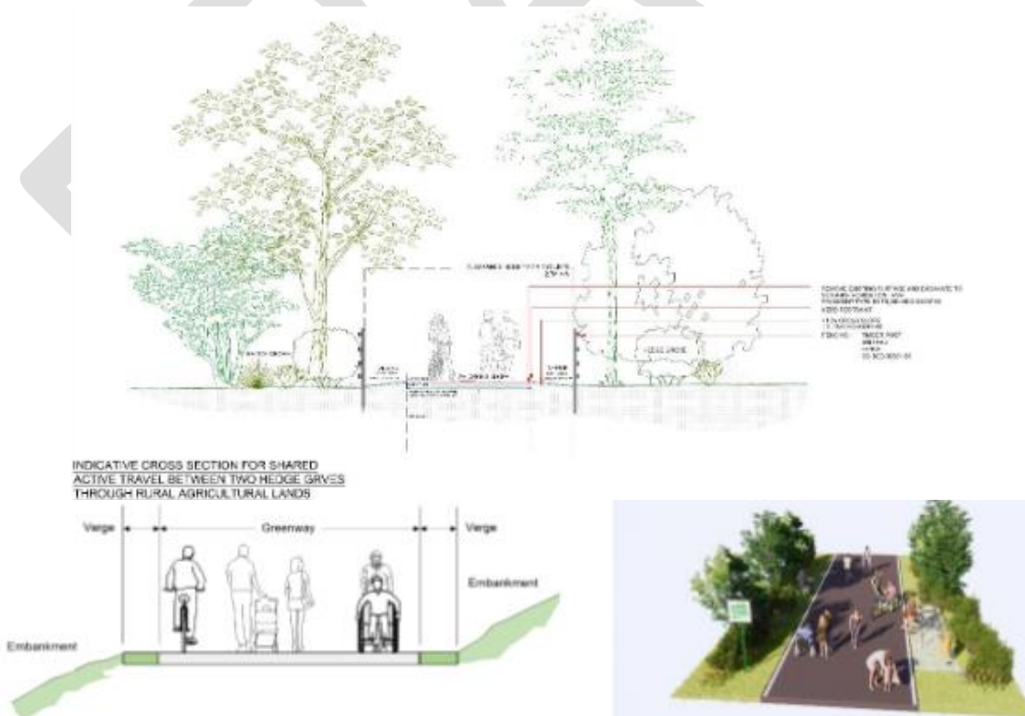
Figure 4-28 Typical Greenway Cross Section (Source: TII DN-GEO-03047 Rural Cycleway Design (Offline & Greenway) February 2025)
