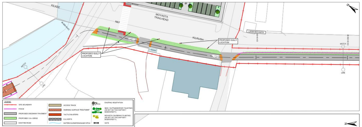
Figure 4-17 Proposed alignment along the N67 at Moyasta
