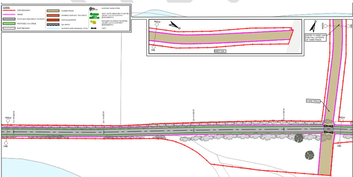
Figure 4-25 Excerpt from Drawing WCGW-ROD-HGN-S1_ML-DR-CH-200541 illustrating the interaction between the Marina Access track, the proposed greenway and the proposed access track for heavy vehicles
